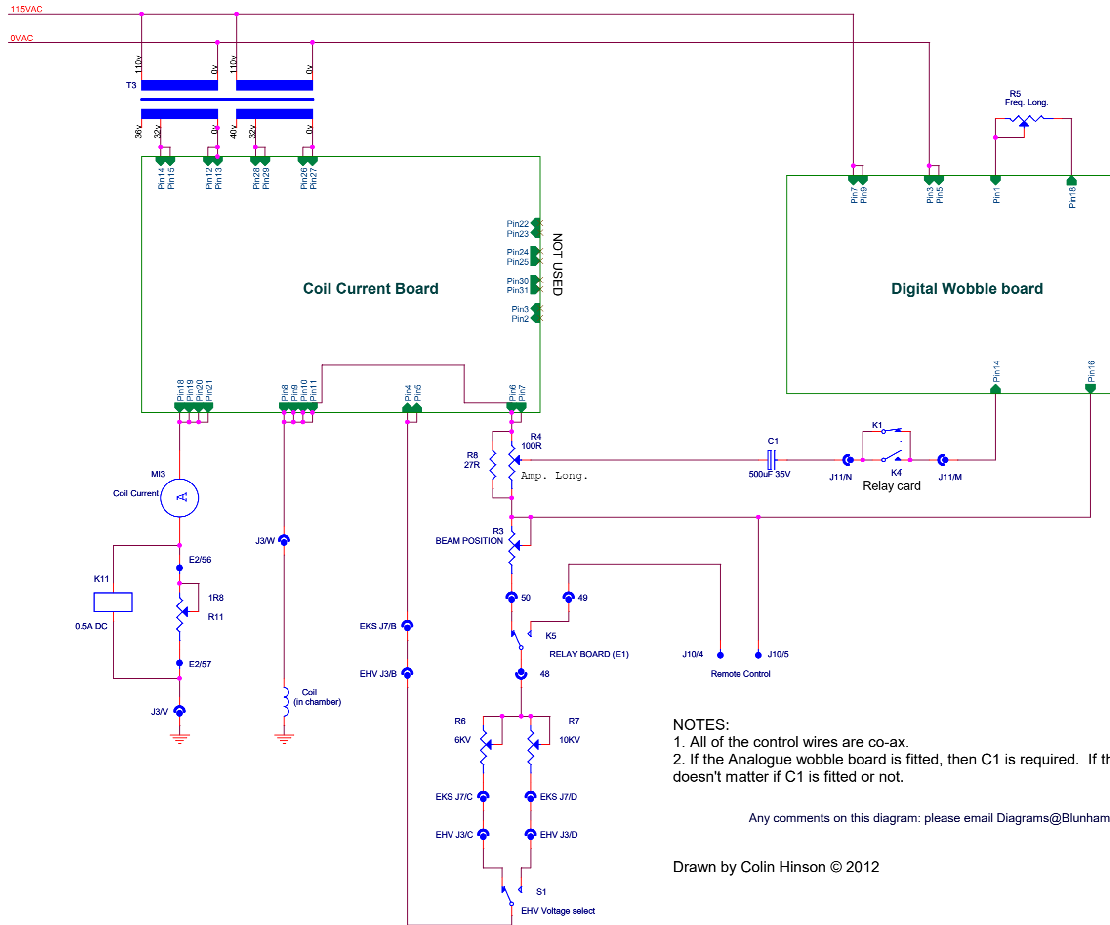
Overall Coil current control diagram for Balzers EKS110 system
