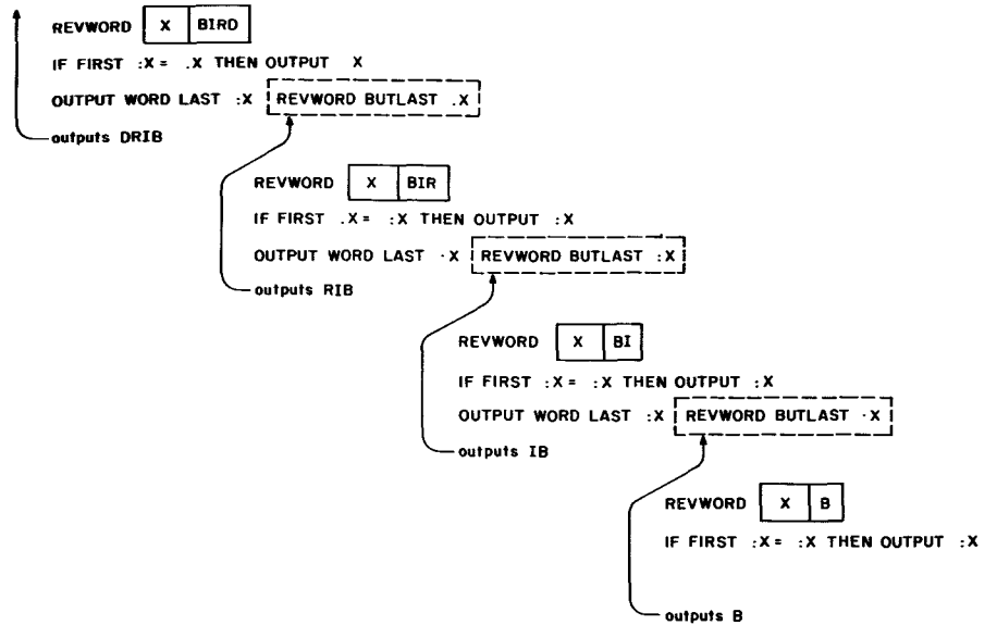
Figure 10.2: Procedure calls in executing REVWORD "BIRD".
