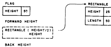
Figure 2.5: Private libraries set up by executing FLAG 50.
