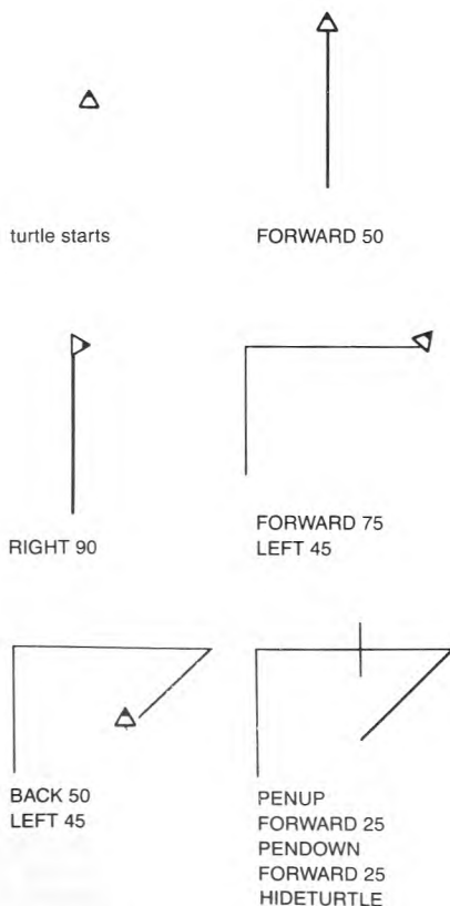
Figure 1.7: Drawing with the turtle.
