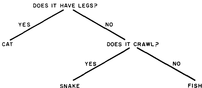
Figure 11.2: Knowledge tree for the ANIMAL program.
