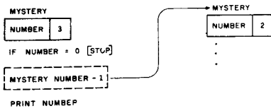
Figure 2.13: Beginning execution of MYSTERY 3.
