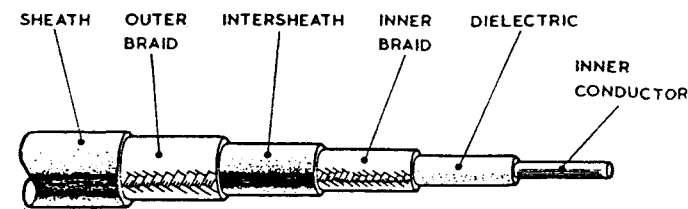
SOLID DIELECTRIC, DOUBLE BRAID, INSULATED
