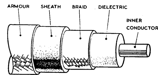
SOLID DIELECTRIC, SINGLE BRAID, ARMoured
