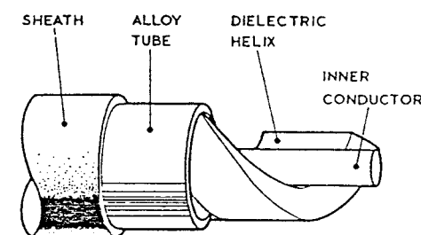
AIR-SPACED, ALLOY TUBE, SHEATHED
