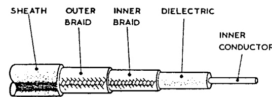
SOLID DIELECTRIC, DOUBLE BRAID
