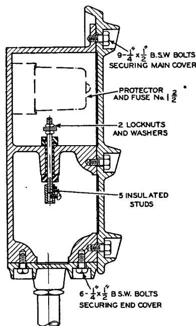
FIG. 7. PROTECTOR AND FUSE UNIT.
