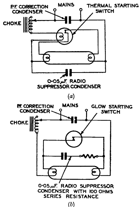
FIG. 4.—TYPICAL LAMP OPERATING CIRCUITS.
