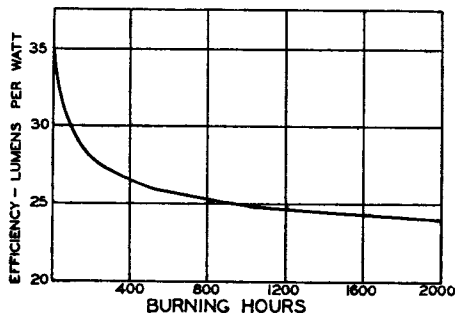
FIG. 5.—TYPICAL EFFICIENCY/LIFE CURVE.
