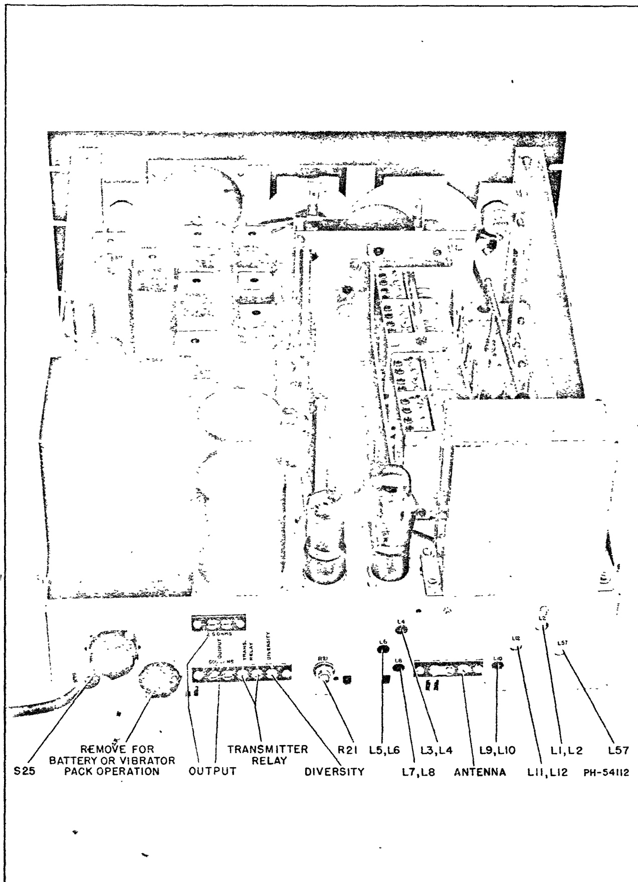
Figure 6—AR-88 Chassis
