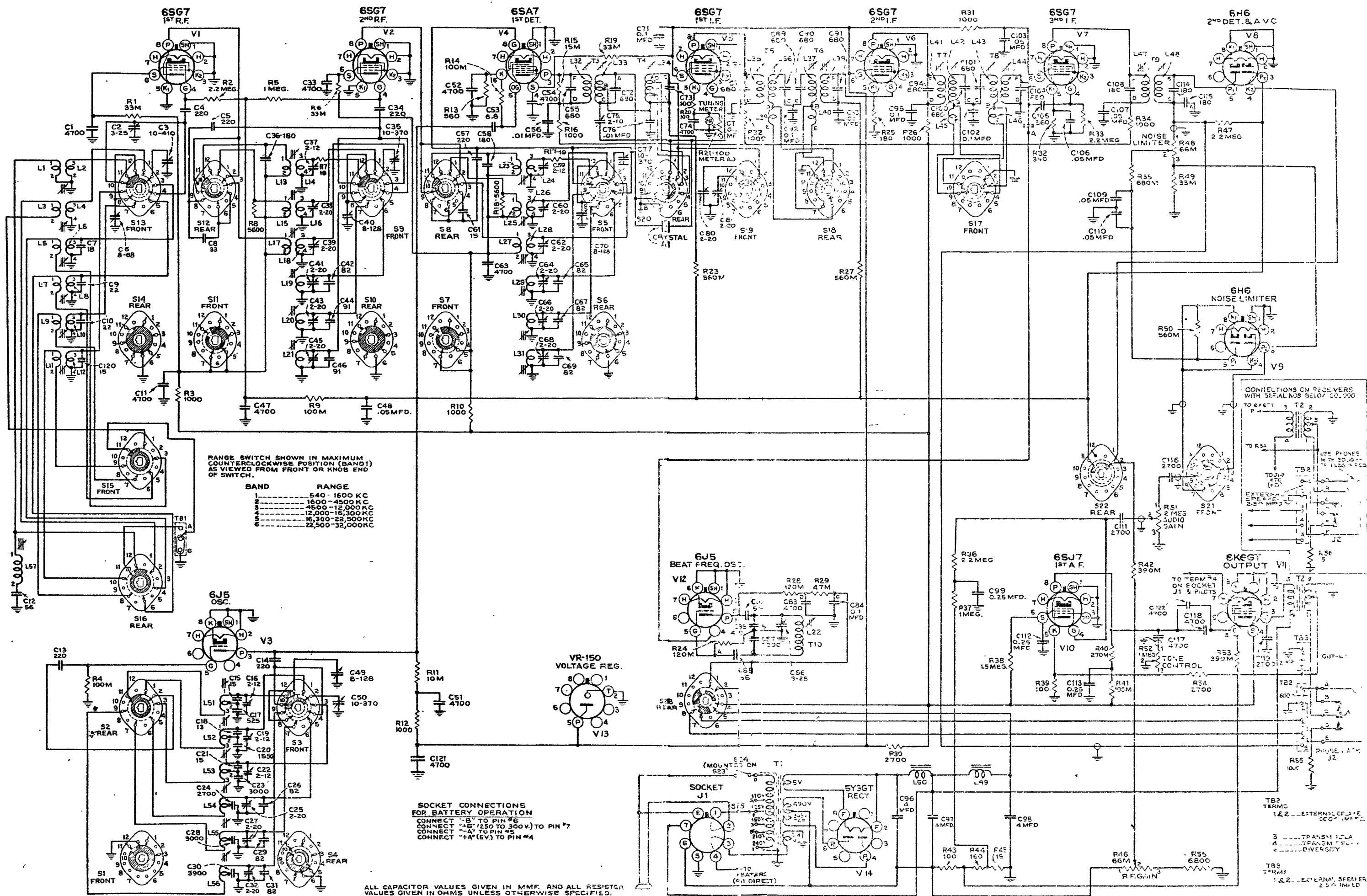
Figure 11—Schematic Diagram
