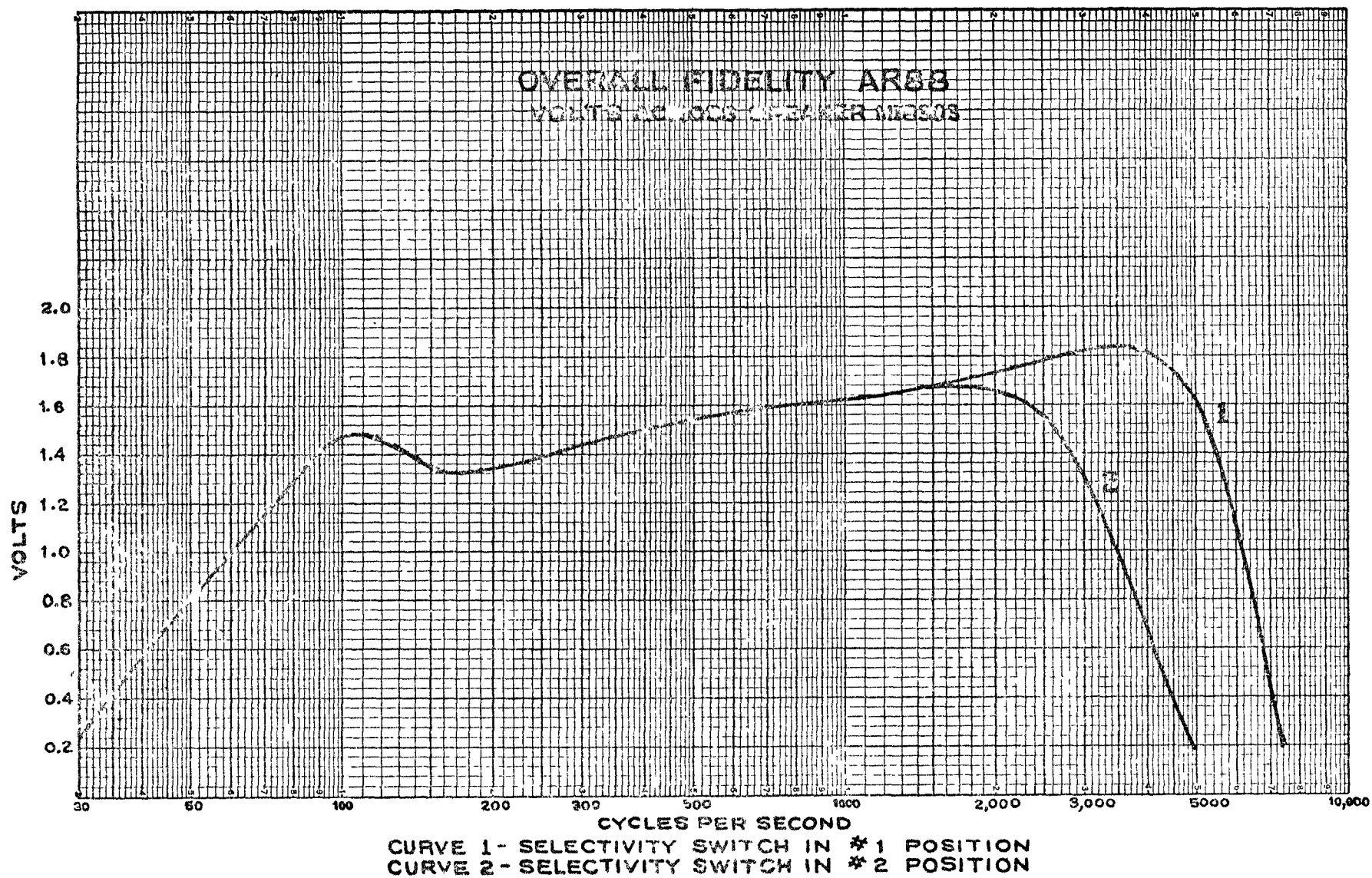
Figure 13—Fidelity Curv
