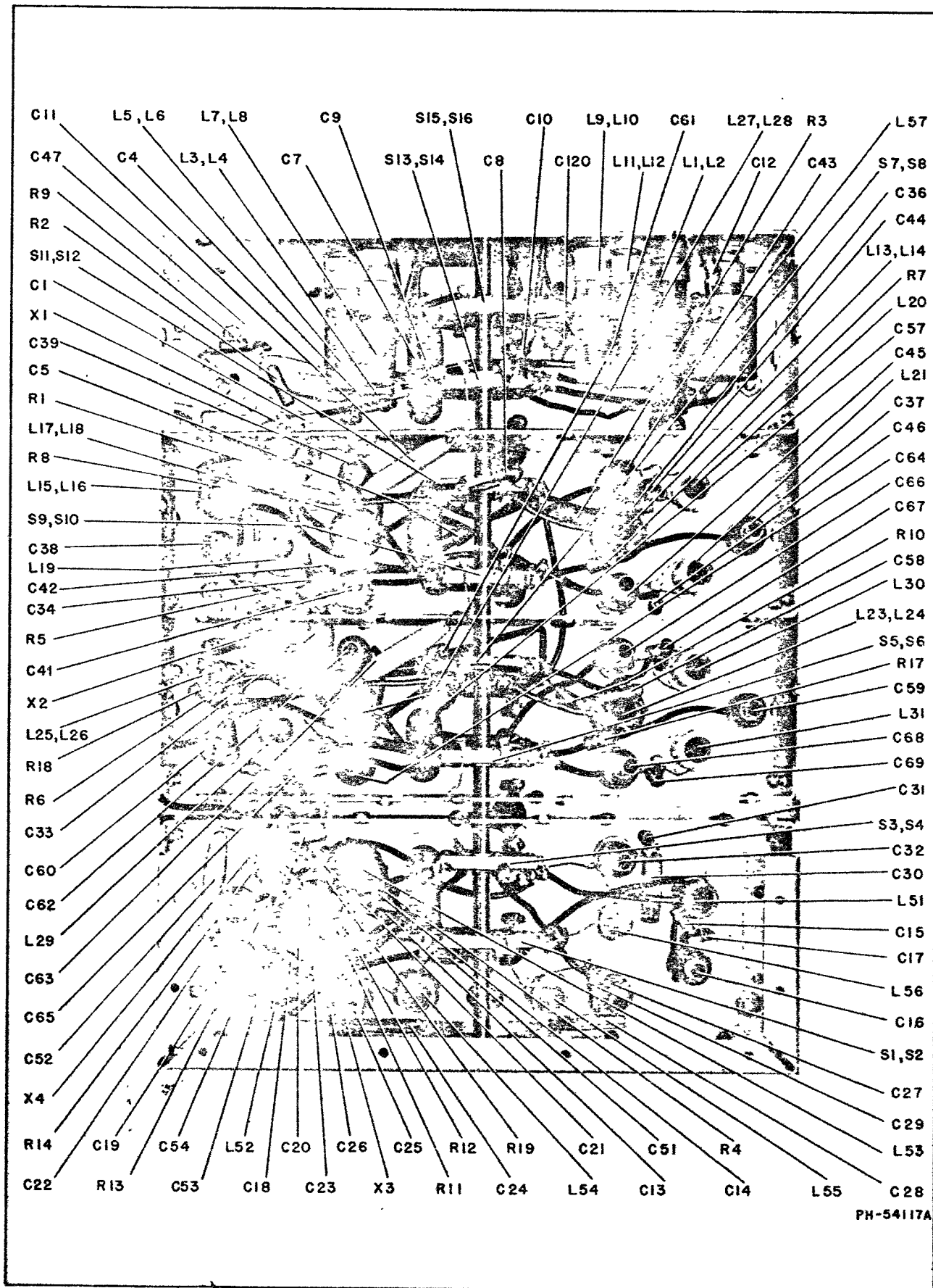
Figure 10—R-F Unit
