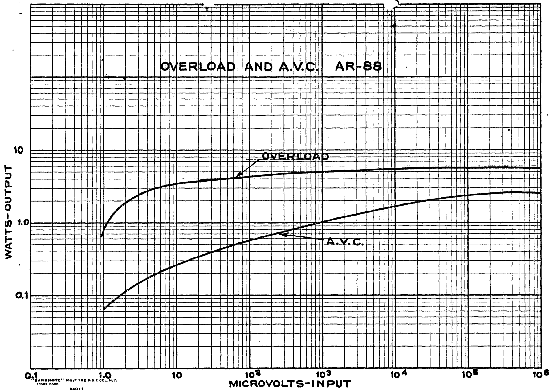
Figure 14—A.V.C. Curves
