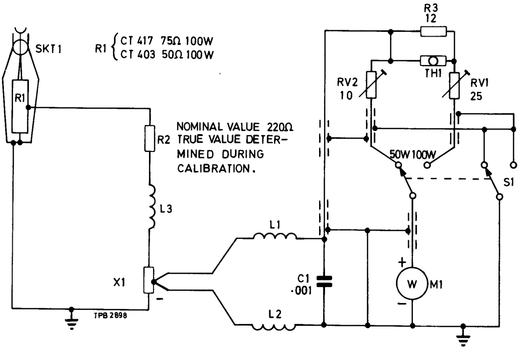
Fig. 5 Wattmeter CT403 and CT417 - modified circuit
