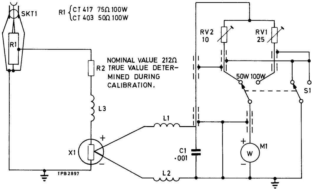
Fig. 4 Wattmeter CT403 and CT417 - old circuit
