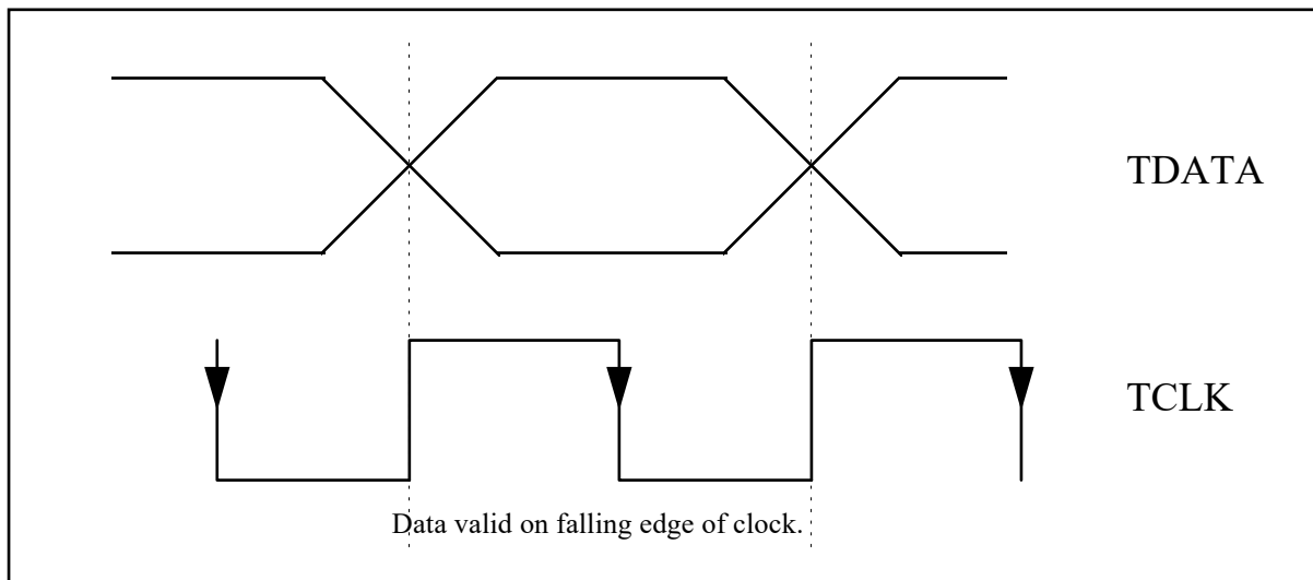
Fig. 7: TDATA and TCLOCK Timing
